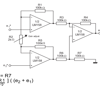
Figure 24: High input Z adjustable gain DC instrumentation amplifier
